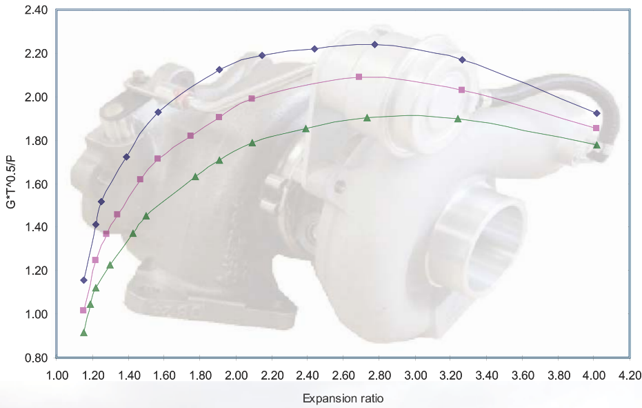
Turbine Maps
